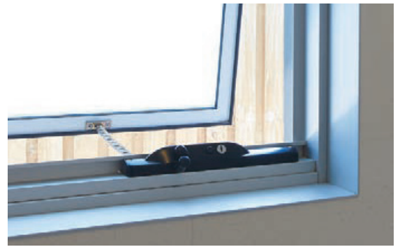
Chain winder with optional sash restriction.
